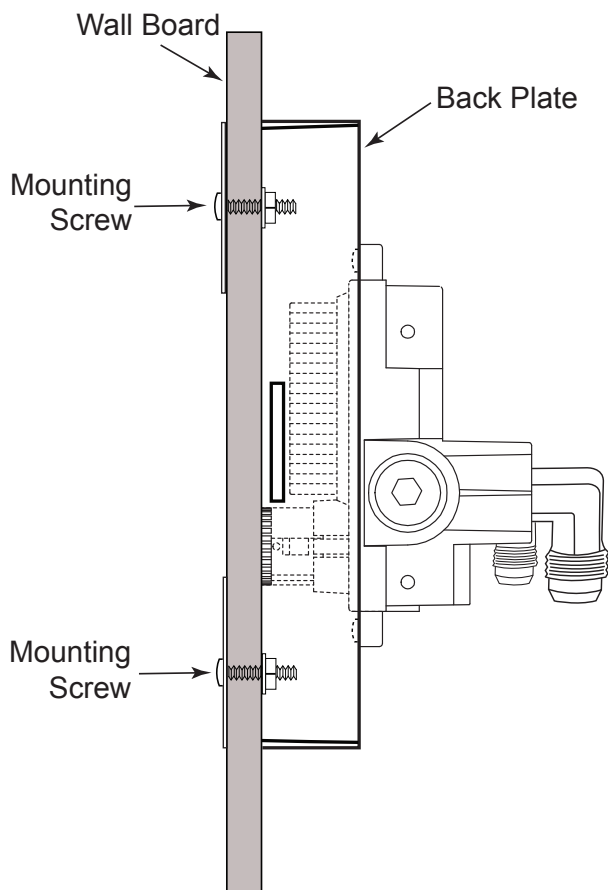
Fig. 4 Side view install of ESTOP with 90° gas fittings.
