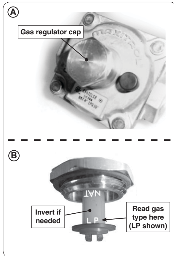
Fig. 26-1 Convert regulator
