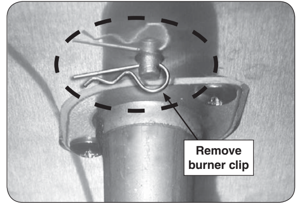
Fig. 30-1 Remove burner clip
