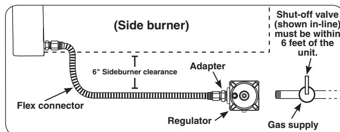
Fig. 18-3 Household propane & natural gas diagram
