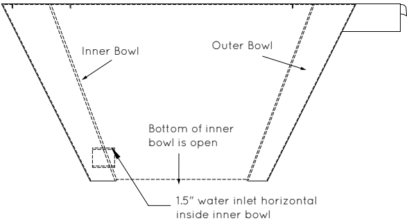
ARTISAN SERIES (SIDE VIEW)
