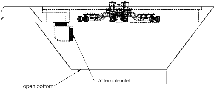
BUILDER SERIES (SIDE VIEW)
