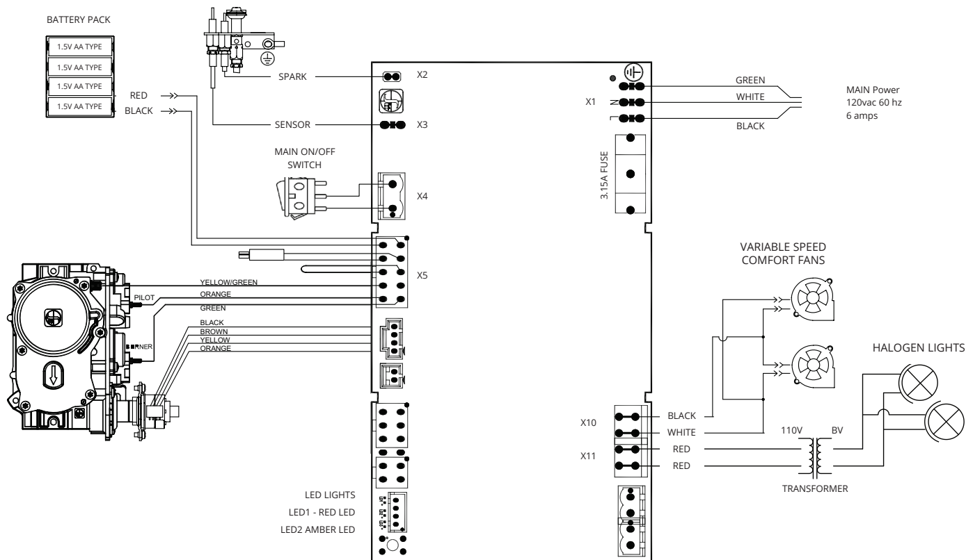
Figure 15b. Wiring diagram for DRSQ38*I-2 with SIT Proflame Electronic Ignition
