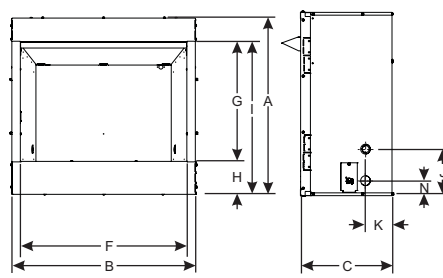
Flush Fireboxes
