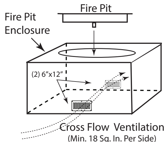
Fig 3. Cross Ventilation Example
