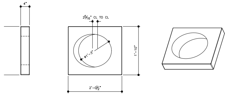
FIGURE 9.3 OFFSET BLOCK
