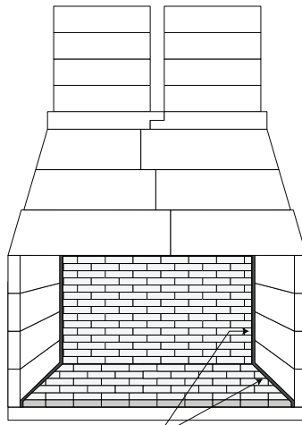
FLOOR & BACK WALL WITH 1/2" EXPANSION GAP ALONG SIDE WALLS
