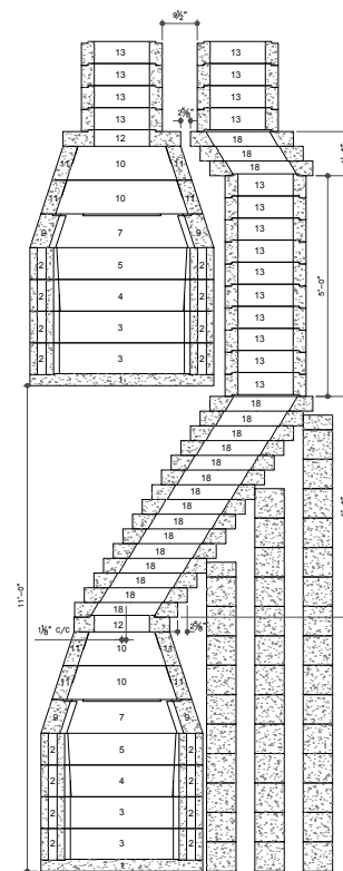
FIGURE 9.4 INSTALLATION WITH OFFSET BLOCKS (SEE FIGURE 14 ON PAGE 34 FOR MORE DETAILS)
