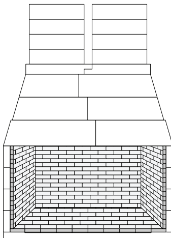
FULLY BRICKED FIREBOX COVERING EXPANSION GAPS
