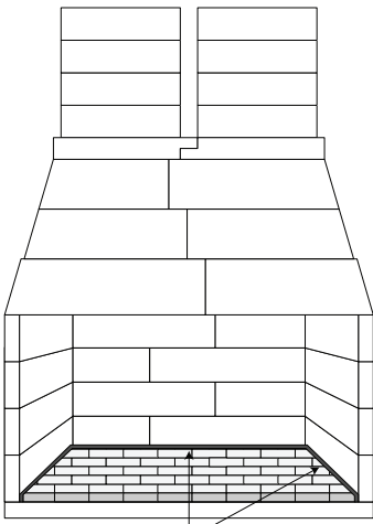
FLOOR WITH 1/2" EXPANSION GAP ALONG BACK AND SIDE WALLS
