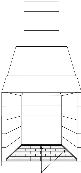
FLOOR WITH 1/2" EXPANSION GAP ALONG BACK AND SIDE WALLS
