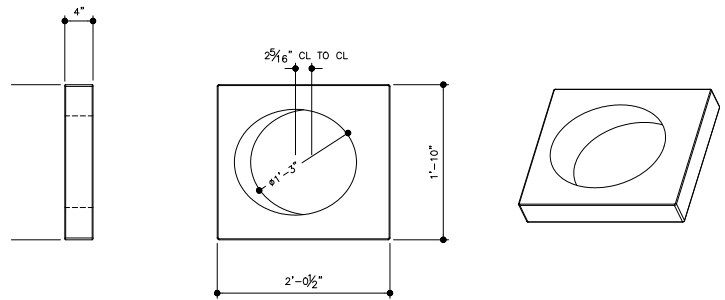
FIGURE 9.3 OFFSET BLOCK
