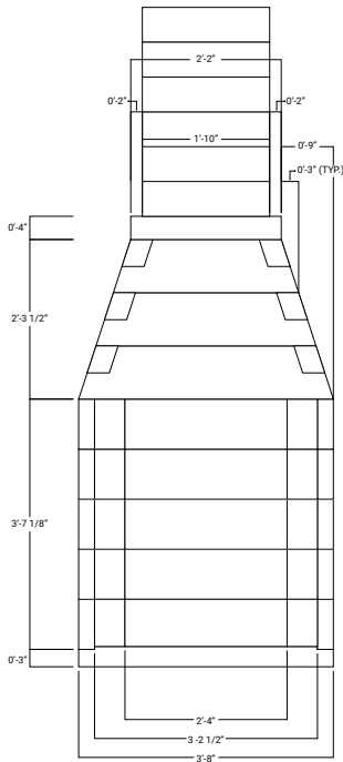
FIGURE 1.2 36" RUMFORD
