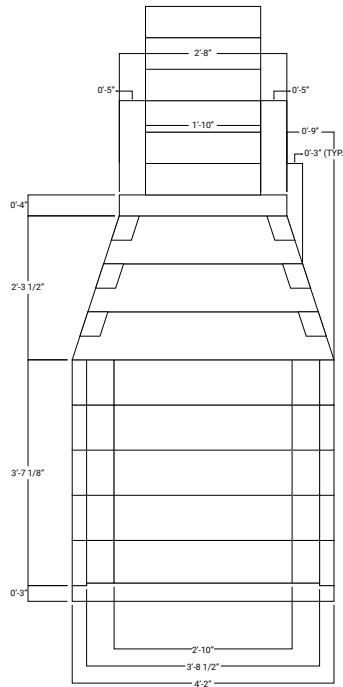
FIGURE 1.3 42" RUMFORD
