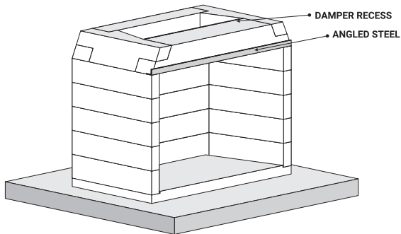
FIGURE 7.2 DAMPER RECESS + ANGLED STEEL
