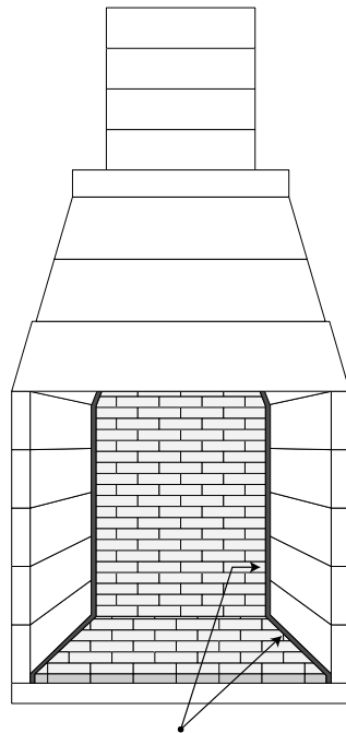
FLOOR & BACK WALL WITH 1/2" EXPANSION GAP ALONG SIDE WALLS
