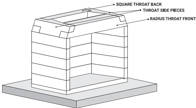
FIGURE 7.1 ASSEMBLED THROAT
