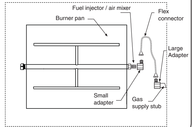
Fig. 7-1 - Fireplace valve
