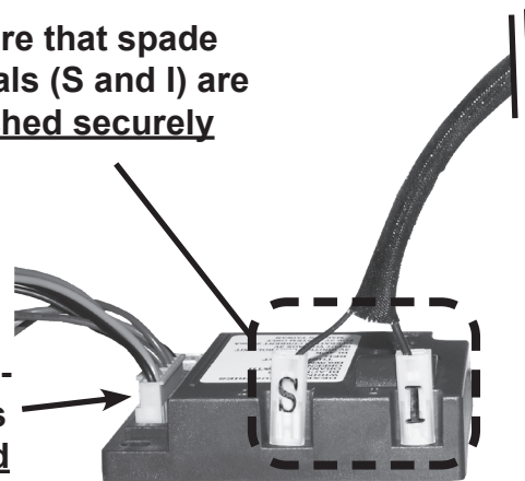
Control Module (DESIGN MAY VARY)
