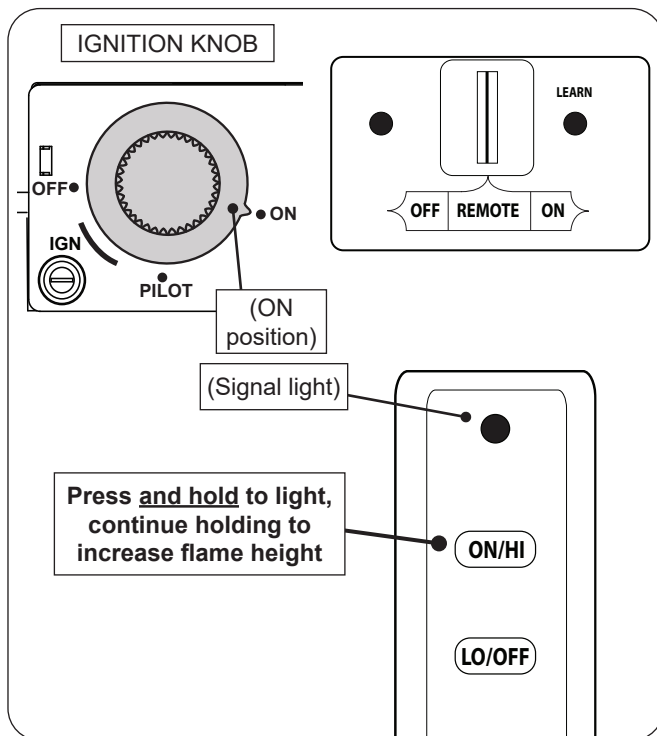
Fig. 28-1 Remote lighting
