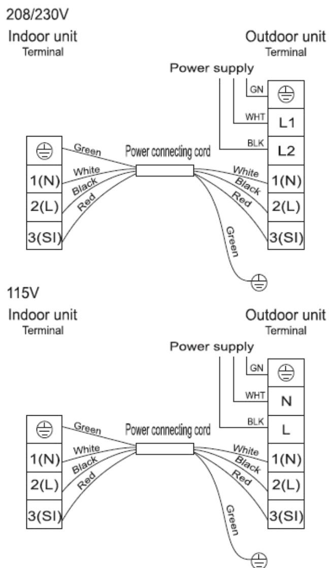
Fig. 4.4b: Wiring Diagram
