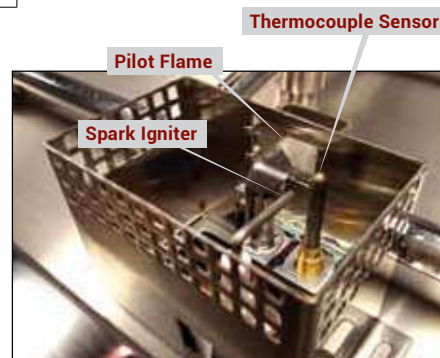
PILOT ASSEMBLY AND BLOWOUT BOX
