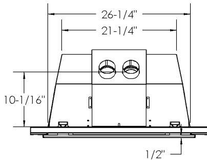
Min. Coverage with Optional I33LK or I33CV
