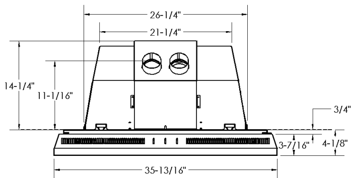
I33CV3 & I33CV5 TOP VOP VIEW
