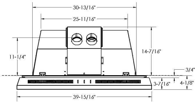
I36CV3 & I36CV5 TOP VIEW
