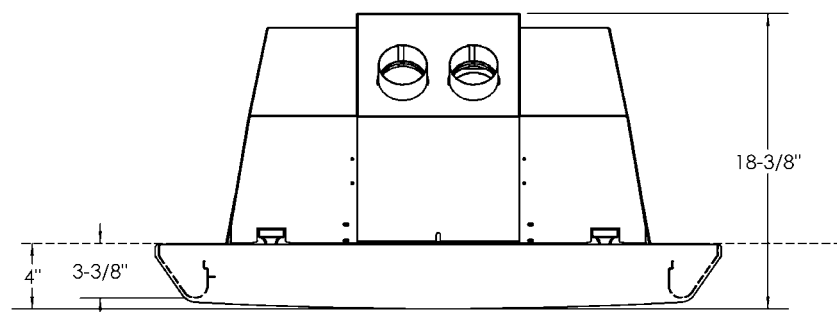
I33LK Kit Top View
