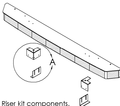
Fig. 3 - Riser kit components.
