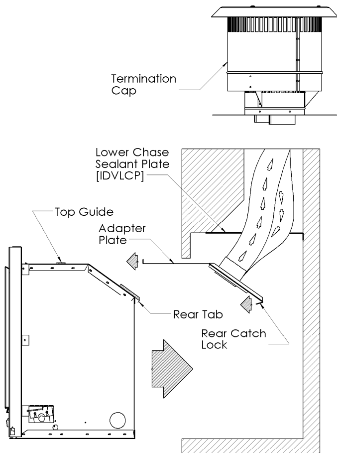
Fig. 2 - Base unit chimney venting install.
