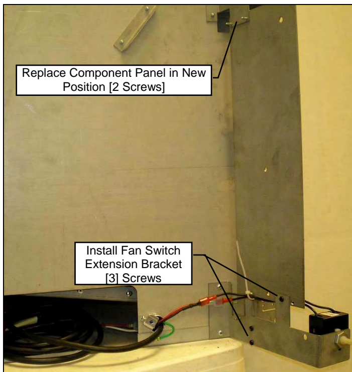
Install Component Panel and Fan Switch Extension in new position.
