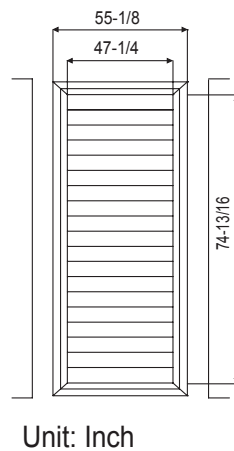
Figure 32: Example of Installing Outdoor Unit Indoors. Louver Dimensions Air Guide Duct on Outdoor Unit
