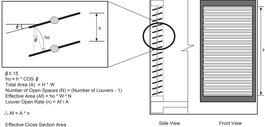
Figure 32: Example of Installing Outdoor Unit Indoors. Louver Dimensions Air Guide Duct on Outdoor Unit
