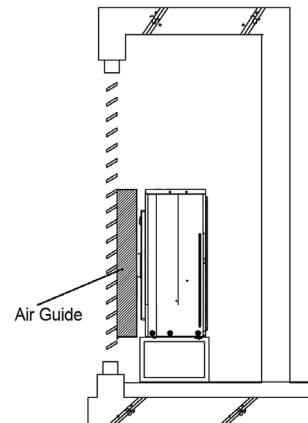
Figure 32: Example of Installing Outdoor Unit Indoors. Louver Dimensions Air Guide Duct on Outdoor Unit
