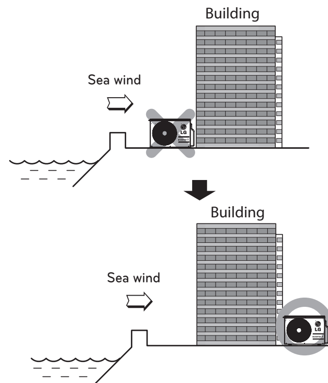
Figure 27: Placement Using Building as Shield.
