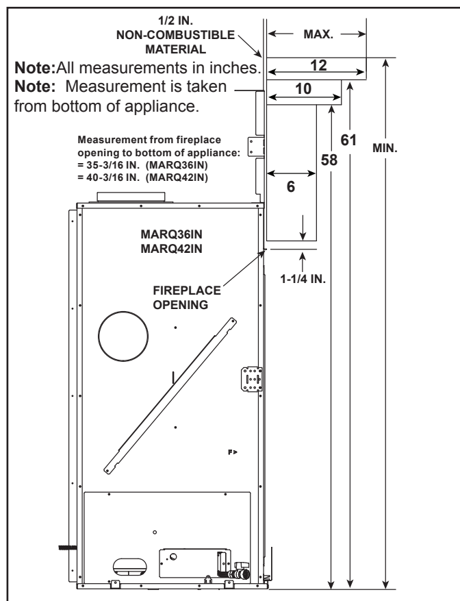
Figure 10.10 Non-Combustible Mantel Allowance - MARQ36IN, MARQ42IN
