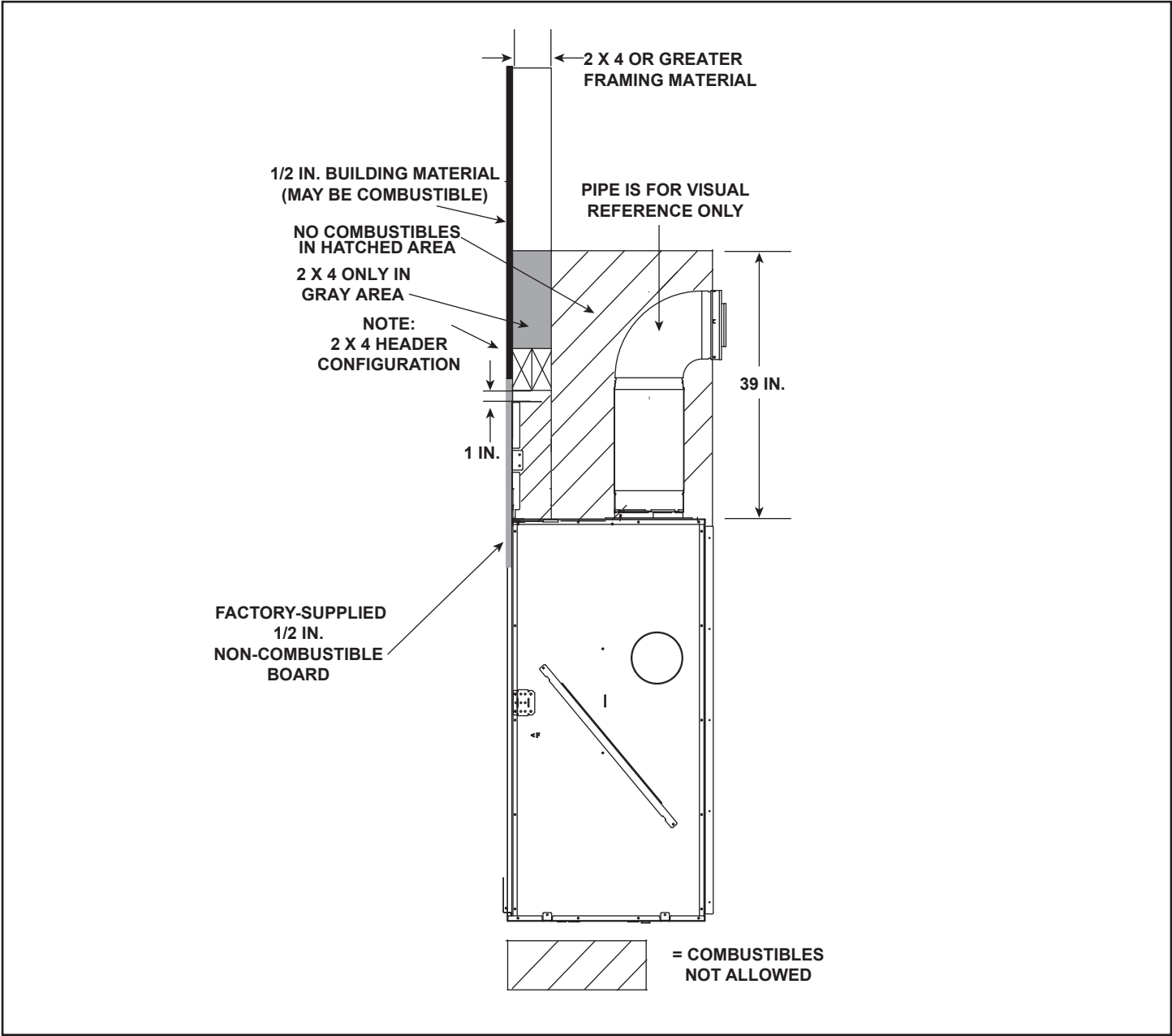
Figure 3.5 Non-Combustible Zone
