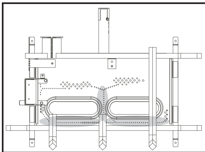
Figure 11.10. Location of Glowing Embers
