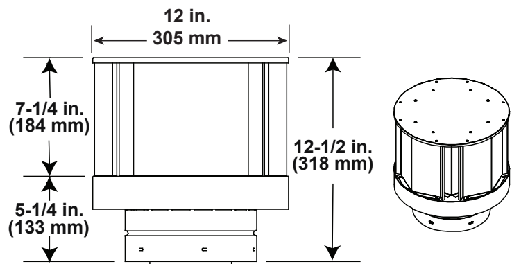
DVP-TVHW Vertical Termination Cap (Highwind)
