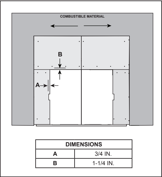
Figure 10.11 Inside Fit Decorative Fronts
