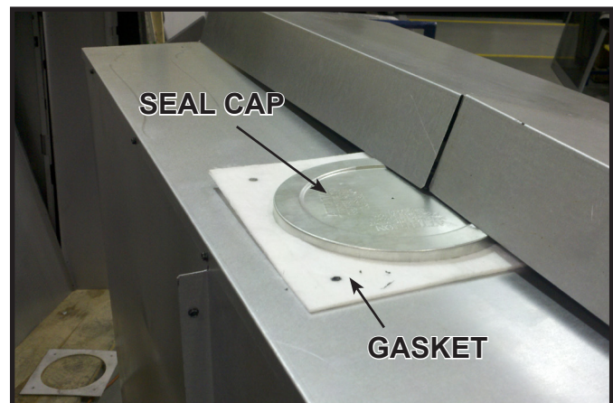
Figure 6.2 Seal Cap and Gasket Location
