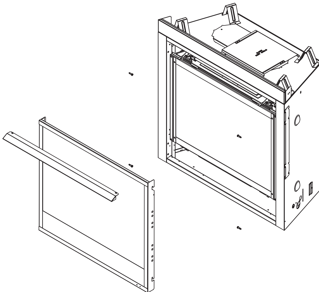
Figure 11.2 Install Majestic Decorative Front and Angled Hood
