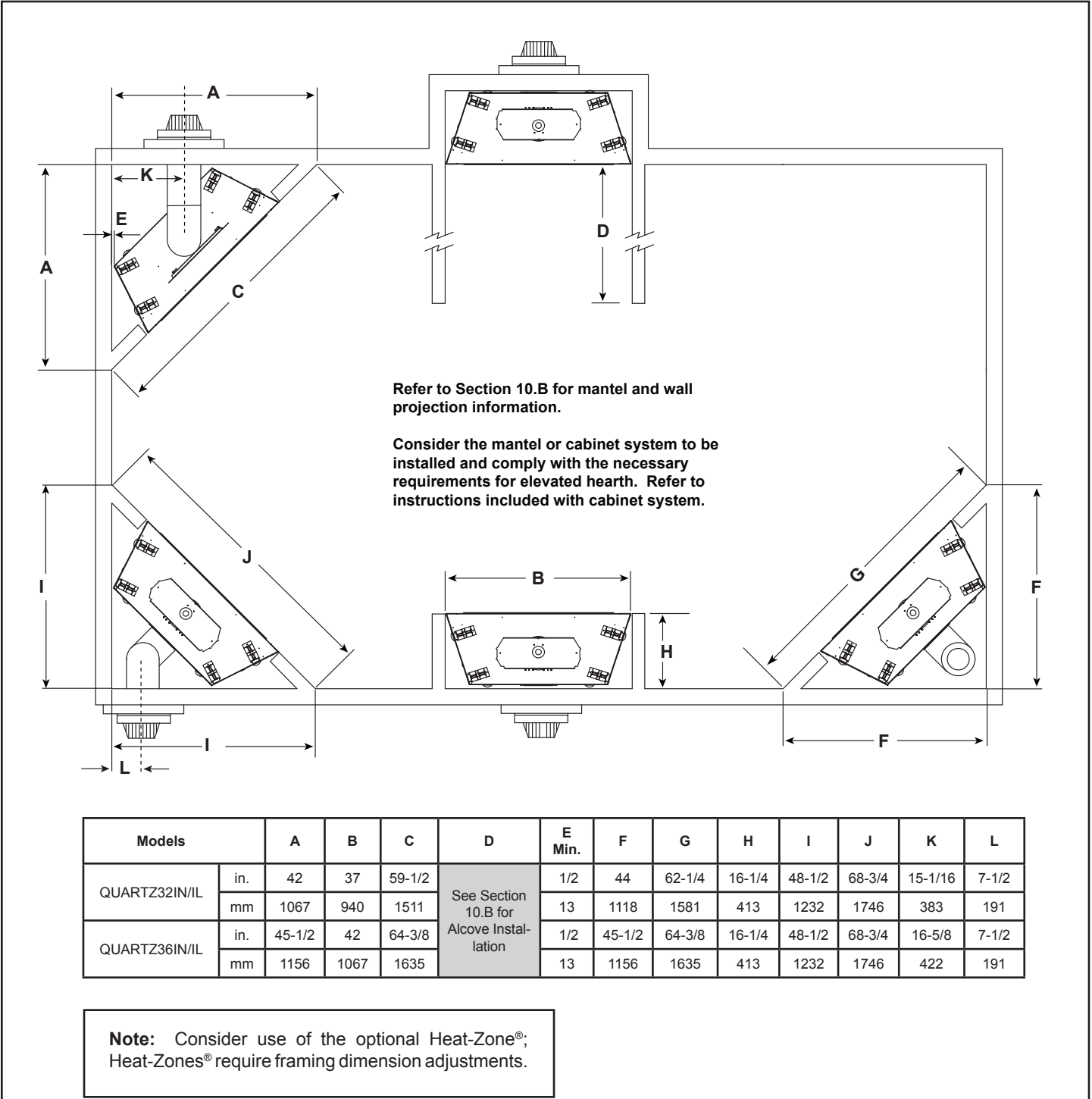
Figure 3.3 Appliance Locations
