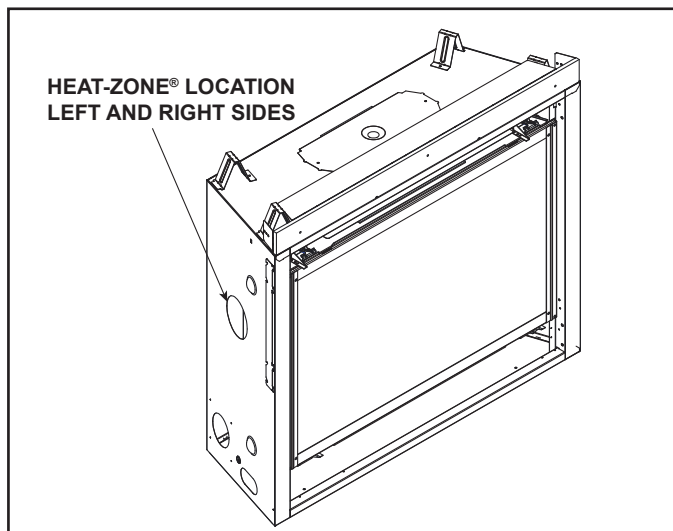
Figure 6.17 Heat-Zone® Locations
