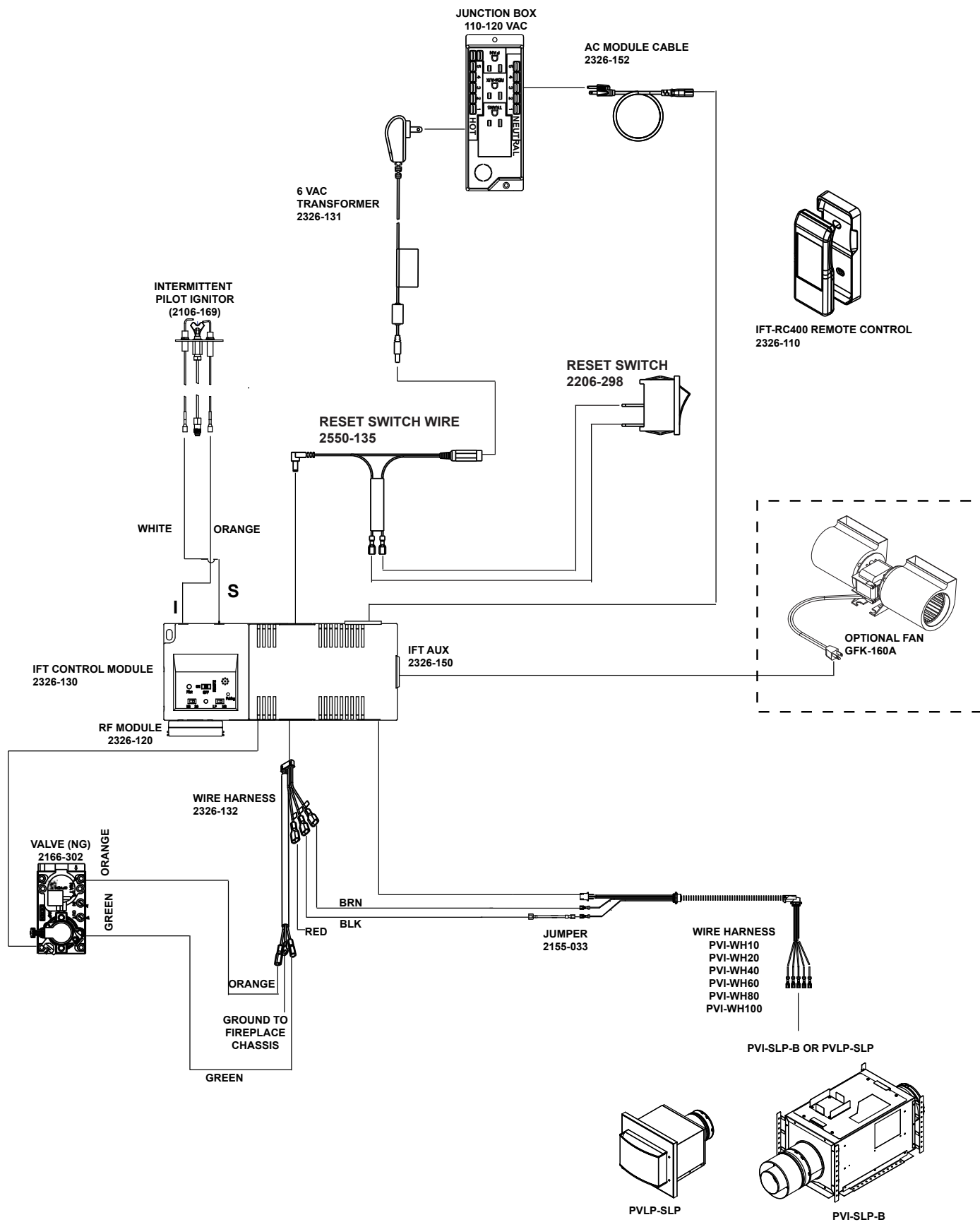
Figure 8.7 Intellifire™ Touch Wiring Diagram with Power Vent Diagram
