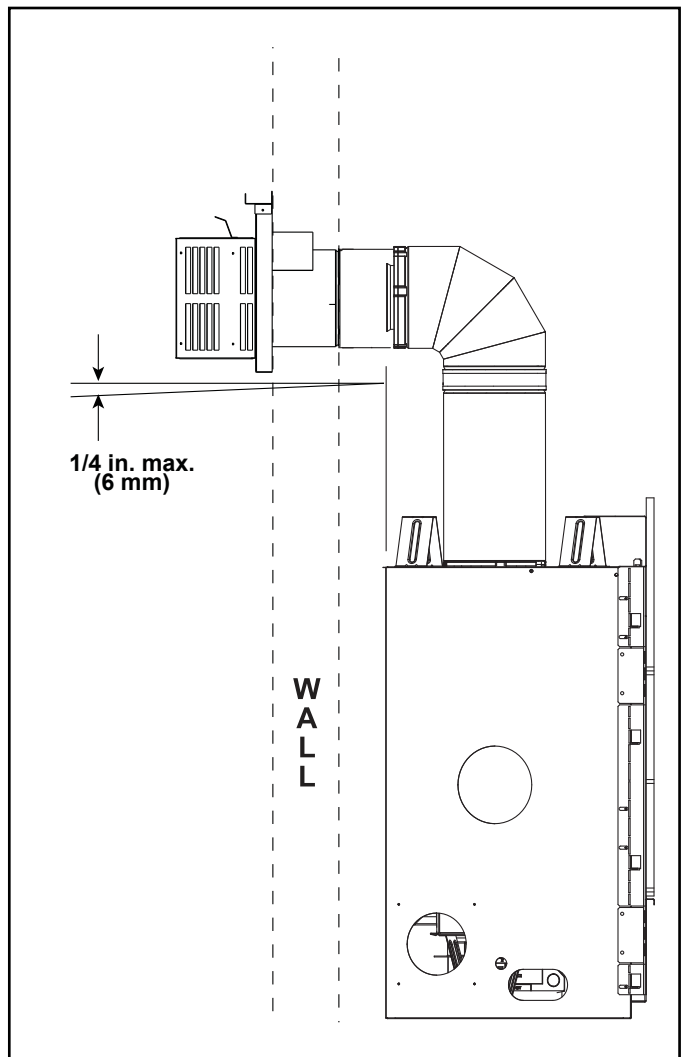
Figure 4.9 Vent Cap
