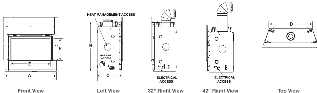
Framing Dimensions
