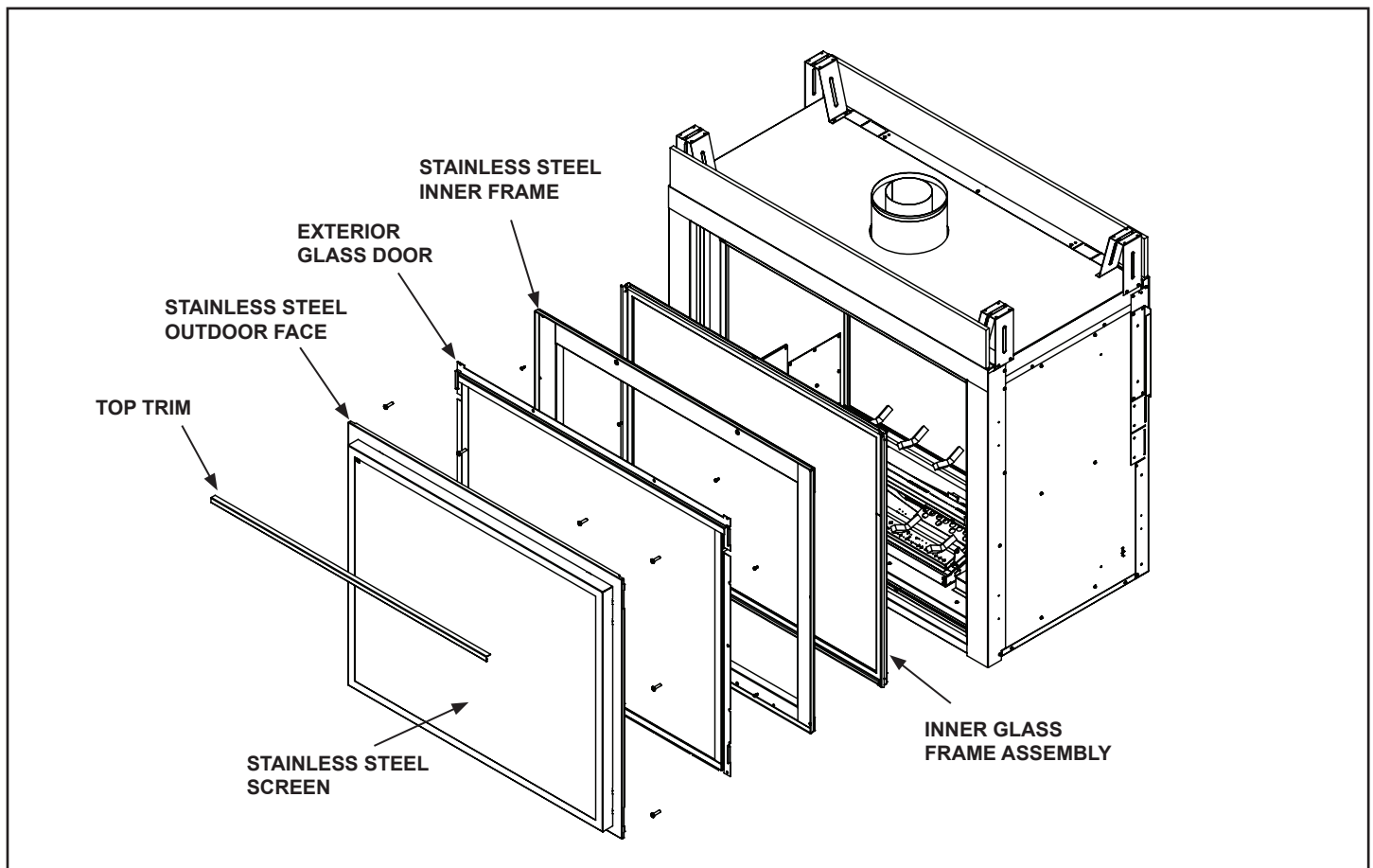
Figure 10.7 Remove Safety Barrier and Glass Frame
