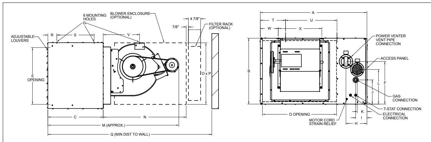
Figure 24.1 - Dimensional Drawings
