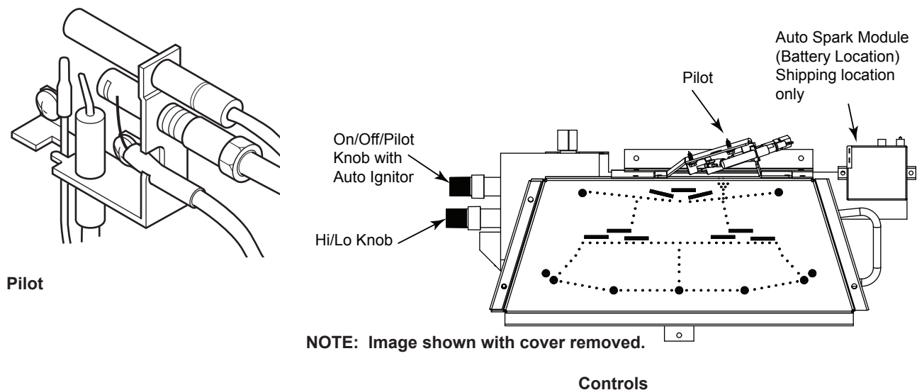
Figure 9.2 - Automatic Ignitor
