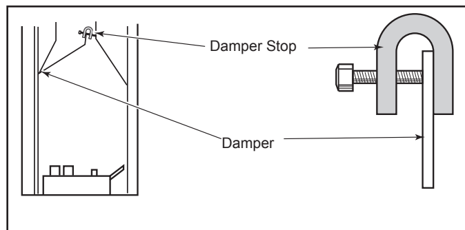
Figure 3.9 - Damper Stop Installation.
