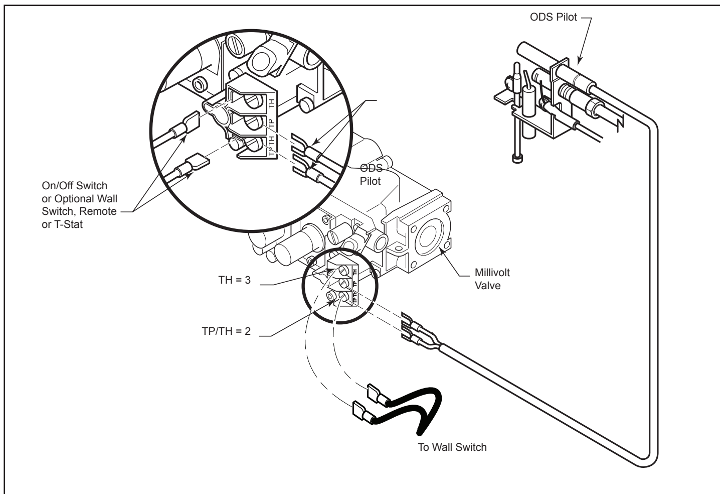
Figure 4.3 - Wiring Diagram
