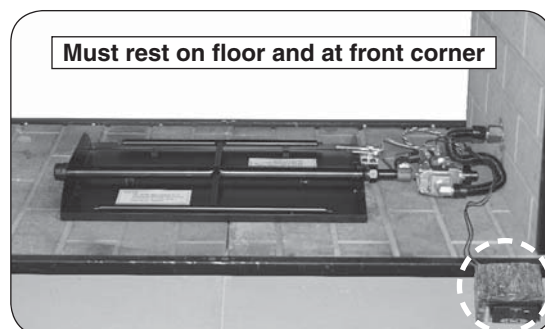
Fig. 19-2 Place heat shield (if applicable)
