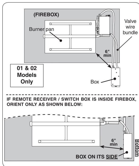
Fig. 18-3 Switch box placement (if applicable)
