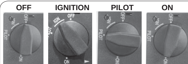
Ignition control knob - positions Fig. 35-1
