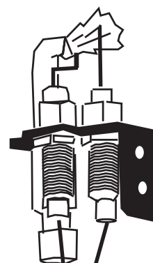
Fig. 31-2 Proper pilot flame
