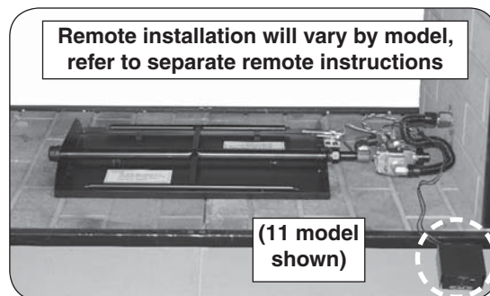
Fig. 19-1 Install remote receiver (if applicable)
