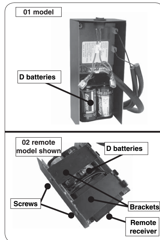
Fig. 24-3 Receiver/switch box batteries
