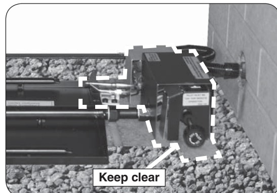
Fig. 20-3 Proper lava media placement
