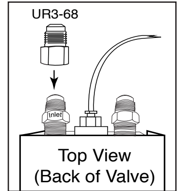
Fig. 2 Installing UR3-68 to the inlet or outlet side of gas valve
