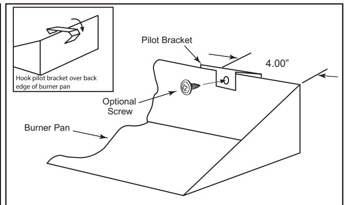
Fig. 4 Pilot Bracket Installation
