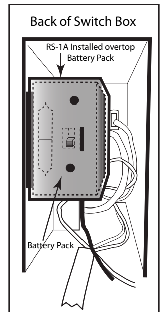
Fig. 11 RS-1A Heat Shield
