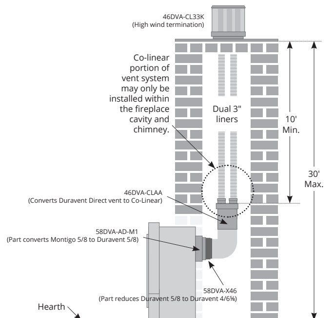
Figure 99.b Co-linear rear vented configuration.
