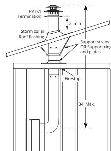
Figure 6.d Side vent, Roof mounted venting (1 = 90° bend).
