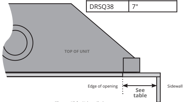
Figure 17.b Sidewall clearances
