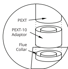
Figure 6. Top vent, roof mounted termination with no offset in vent run.
