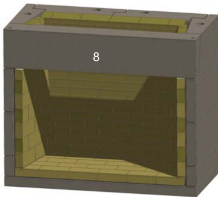
Figure 11. Front Lintel
