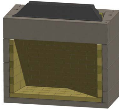
Figure 13. Damper Placement
