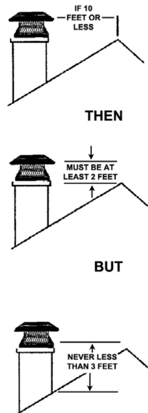
Figure 26. Chimney Height
