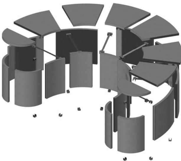
Exploded View
