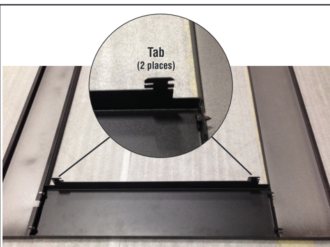
Figure 2 - Tabs Positioned to the Inside
