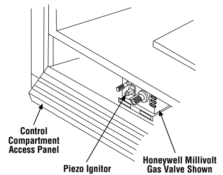
Control Compartment Access - Millivolt Control Valve Shown
