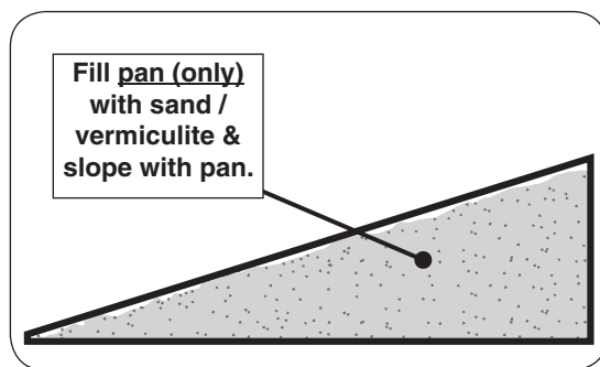
Fig. 14-4 Sand/vermiculite detail
