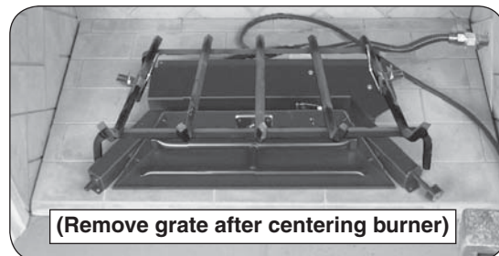
Fig. 13-3 Position grate
