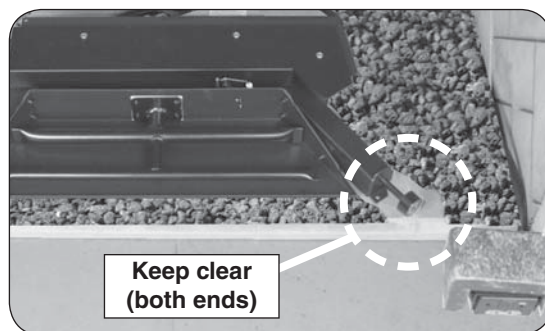
Fig. 14-2 Proper lava granules placement
