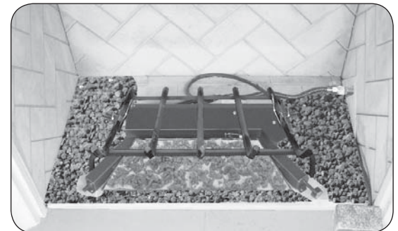
Fig. 15-3 Place grate
