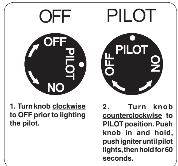
Fig. 19-1 Control knob detail (OFF, PILOT)
