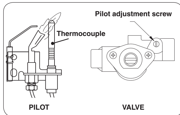
Fig. 23-1 Pilot adjustment detail
