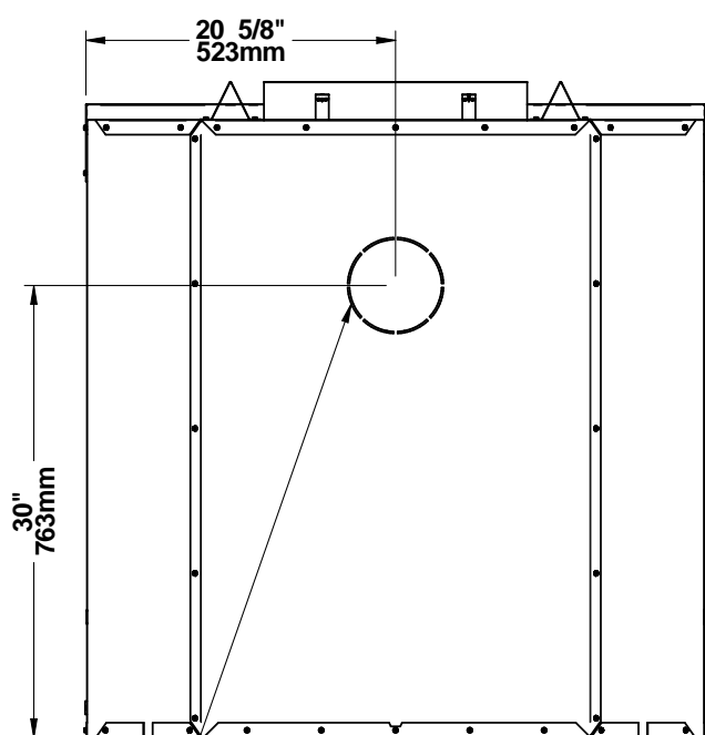
ENSEMBLE D'AIR PULSÉ 6"/152mm (3) 6"/152mm FORCED AIR KIT (3)
