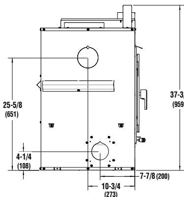
Figure 11 - Framing Dimensions
